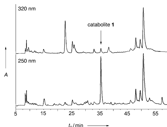
Figure 1. HPLC analysis of an extract of senescent leaves of Norway maple. The catabolite 1 gives rise to a strong signal at 250 nm and a weak one at 320 nm (where NCCs have a characteristic absorption). [8]
