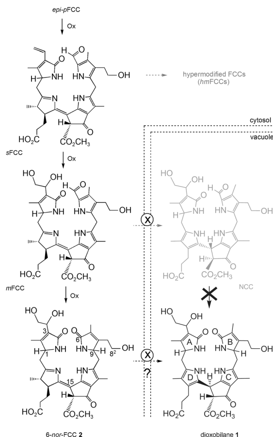
Scheme 2. Structural outline of the proposed later part of chlorophyll in senescent leaves of Norway maple ( Acer platanoides ), which begins with a “primary” FCC, deduced to be epi-pFCC (the C-1 epimer of pFCC). [25] Hydroxylation at C-8 2 , followed (in an unknown sequence) by dihydroxylation of the vinyl group at C-3 and oxidative deformylation at C-6, probably furnishes the still-elusive 6-nor-FCC 2 in the cytosol. The catabolite 1 may be formed in the vacuole by a hypothetical isomerization of 2 and transport of 2 into the vacuole by the catabolite transporter X. Hypermodified FCCs (hmFCCs, found in bananas) [29] and NCCs, as found in senescent leaves of barley [6] , were not detected in the leaves of Norway maple.
