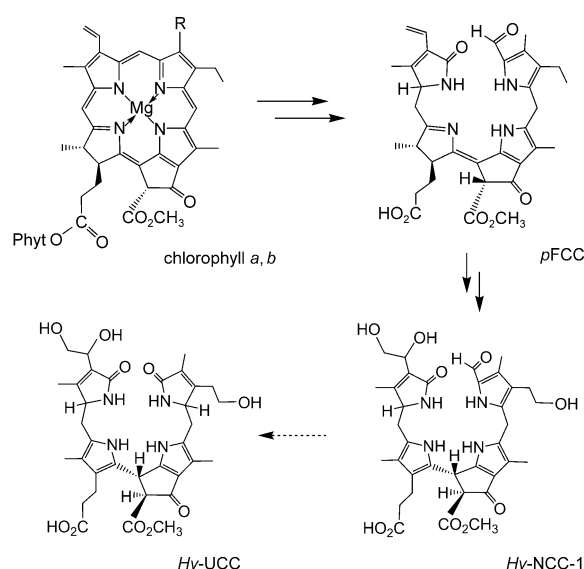
Scheme 1. Short outline of chlorophyll breakdown represented by the structures of catabolites identified in barley ( Hordeum vulgare ). [6,7] Chlorophyll a (R = CH 3 ) and b (R = CH=O) are broken down in senescent chloroplasts to the primary FCC (pFCC). pFCC is modified by enzymes in the cytosol and the resulting mFCCs are exported into the vacuole, where NCCs (such as Hv -NCC-1) are formed by chemical isomerization. Hv -UCCs were detected in barley leaves and were suggested to be oxidation products of Hv -NCC-1. [10]
